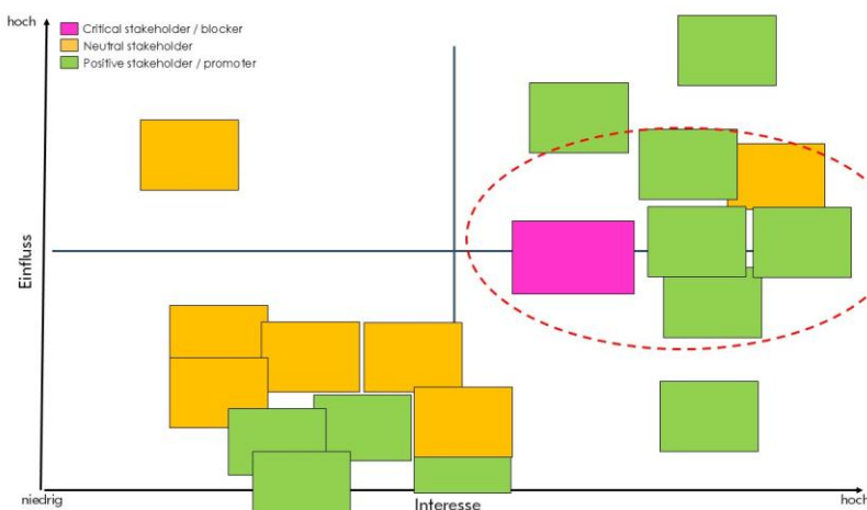
Figure 25: Exemplary stakeholder matrix, Source: StadtLabor
