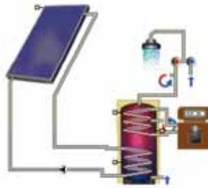
Figure 50: Hydraulic scheme of the DHW system for multifamily houses
