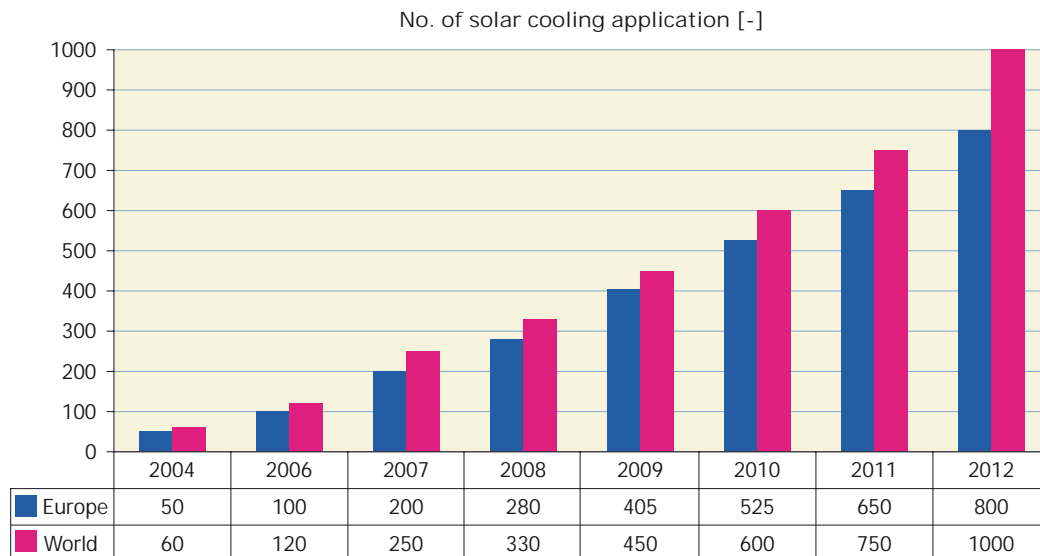
Figure 46: Market development of small to large-scale solar air conditioning and cooling systems (Source: Solem Consulting / Green Chiller)
